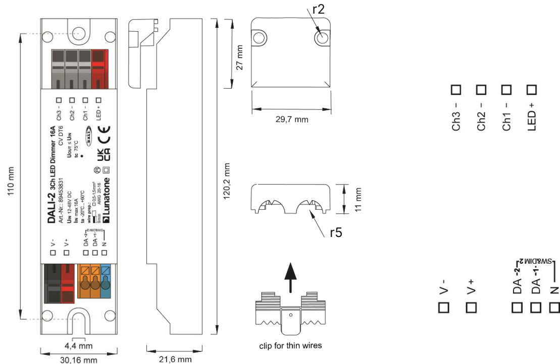
dimensions remote ceiling Version 16A Art.Nr.: 89453831 Version 10A Art.Nr.: 86459571
